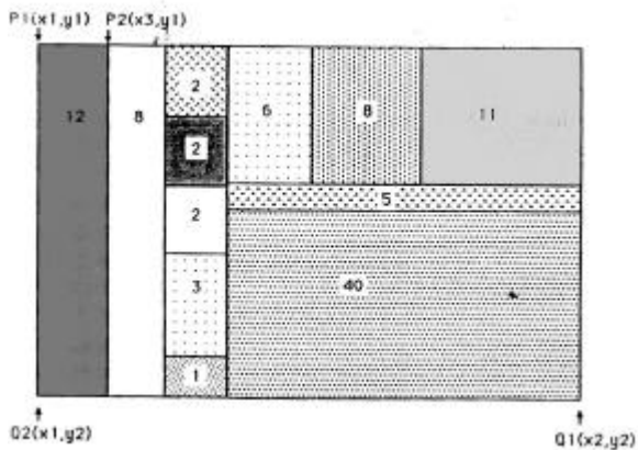
Gambar 2. Implementasi Tree map
