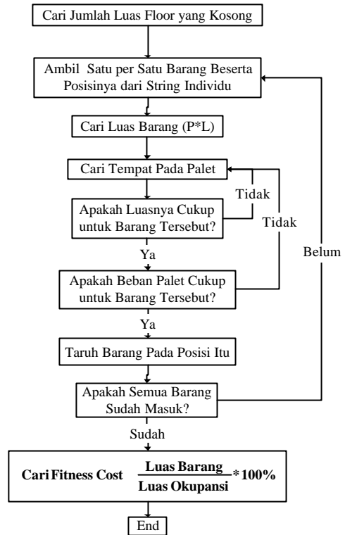
Gambar 14. Algoritma Pencarian Fitness Cost
