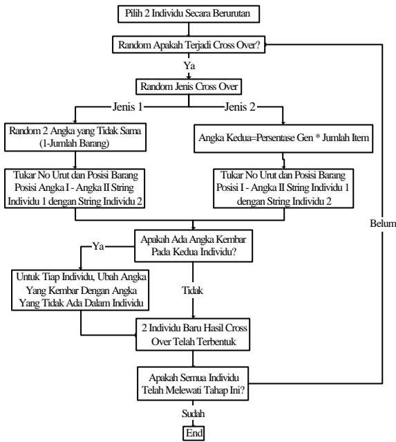
Gambar 16. Algoritma Cross Over
