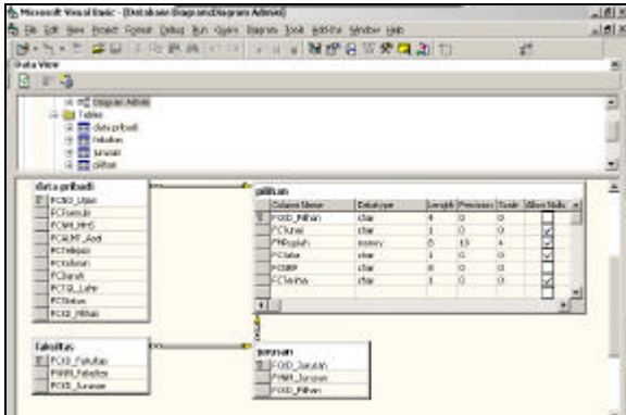
Gambar 6. Database Diagram
