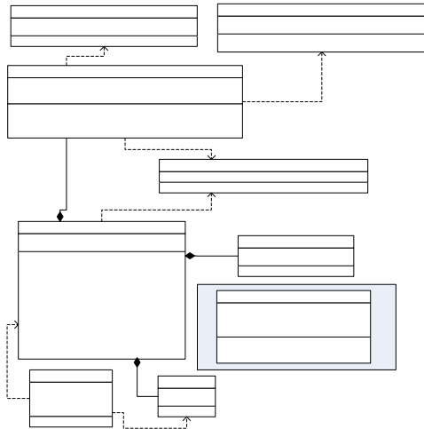
Figure 4. The Model Framework for Compact Version
